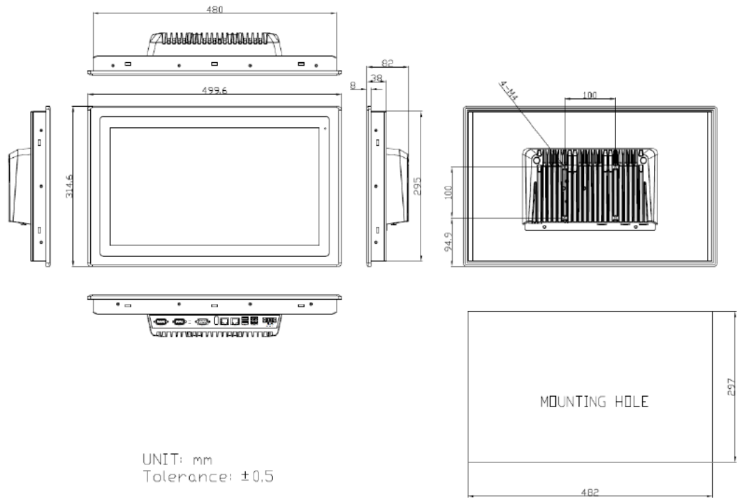
Figure 7 Dimensions of TP-7045-18
