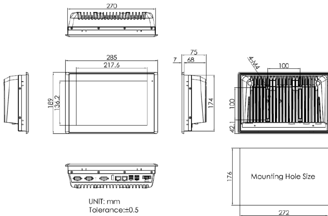
Figure 1 Dimensions of TP-7045-10
