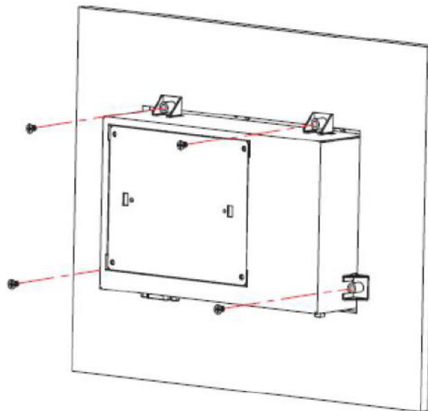
Figure 14 TP-7045 PANEL Mounting
