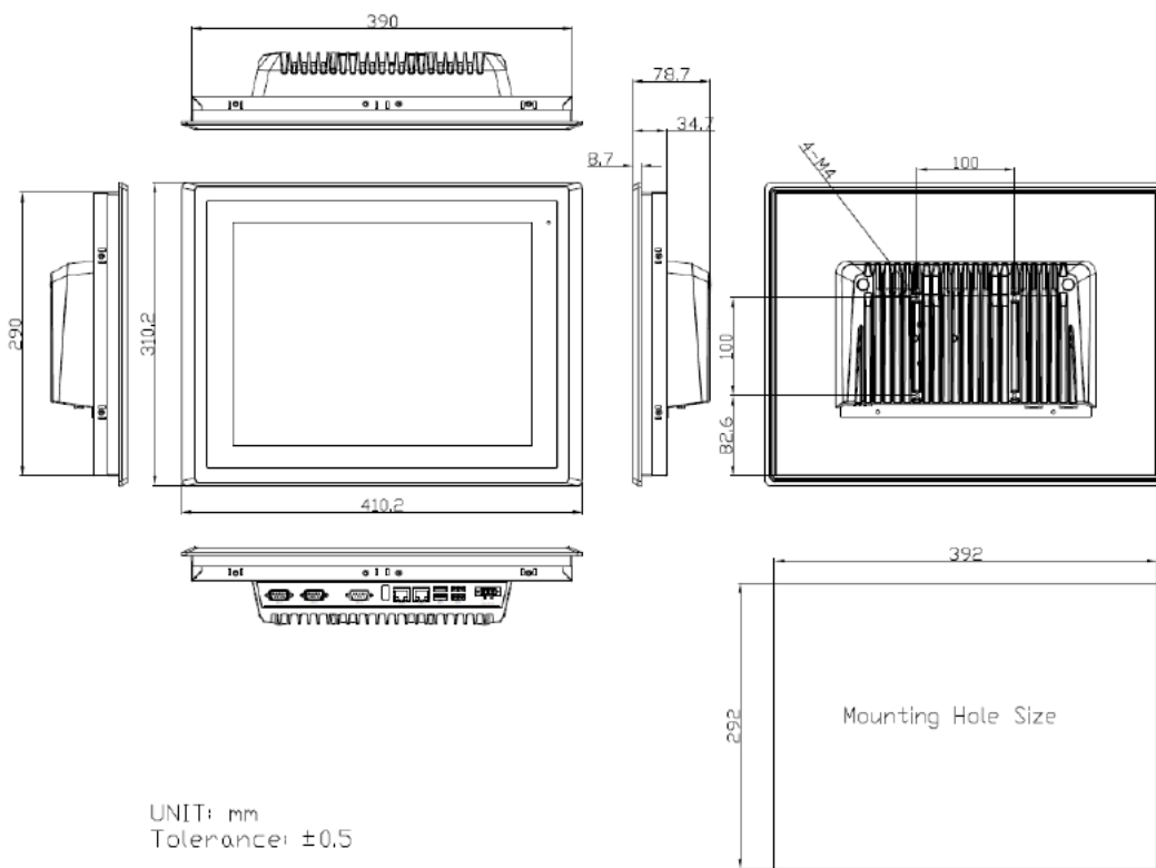
Figure 4 Dimensions of TP-7045-15
