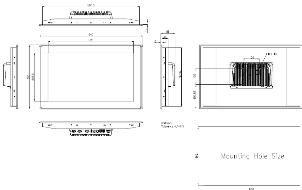
Figure 10 Dimensions of TP-7045-24
