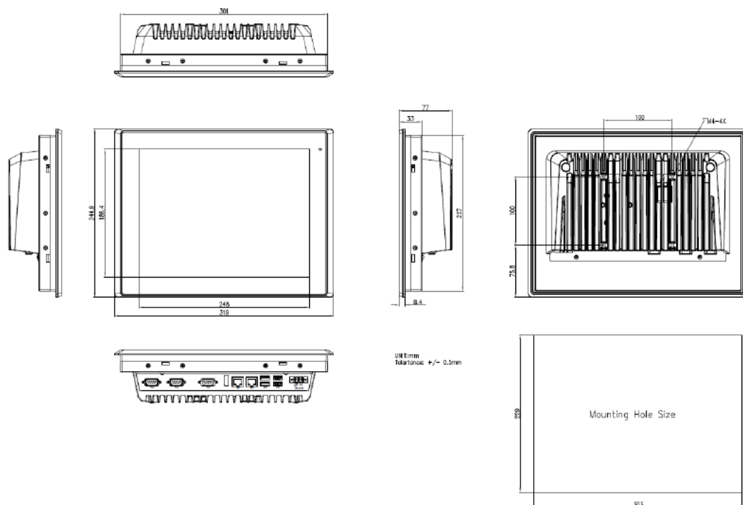
Figure 2 Dimensions of TP-7045-12
