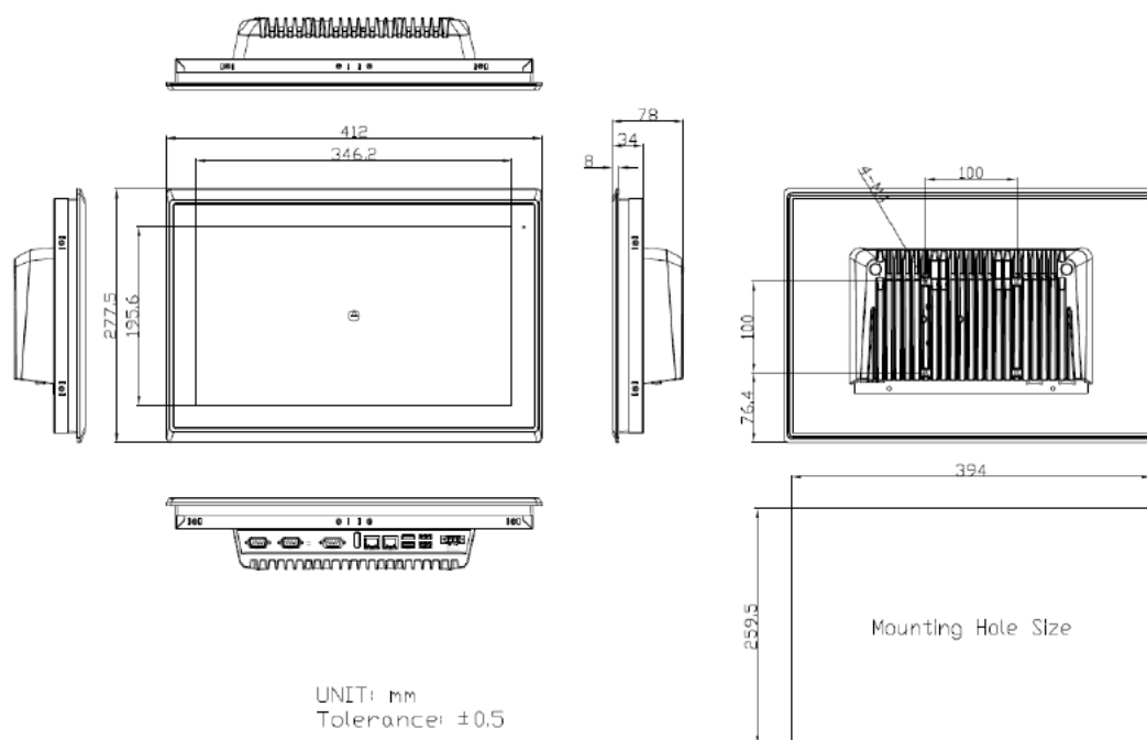
Figure 5 Dimensions of TP-7045-16
