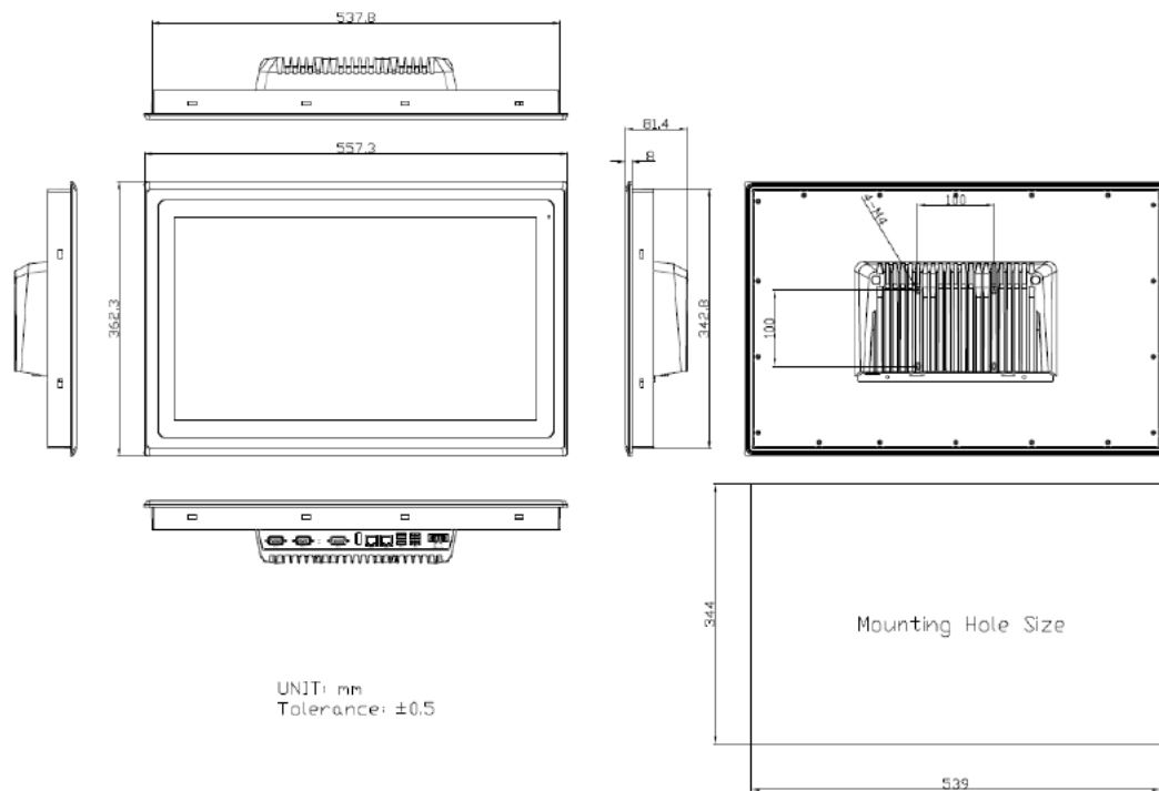
Figure 9 Dimensions of TP-7045-22
