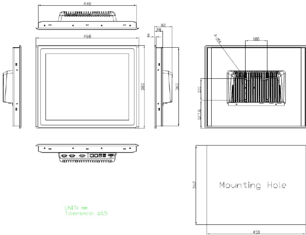
Figure 8 Dimensions of TP-7045-19
