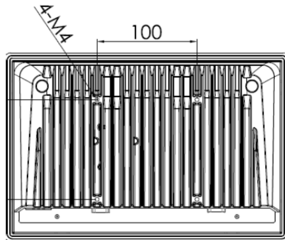
Figure 13 TP-7045 VESA Mounting
