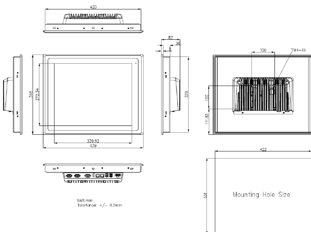
Figure 6 Dimensions of TP-7045-17
