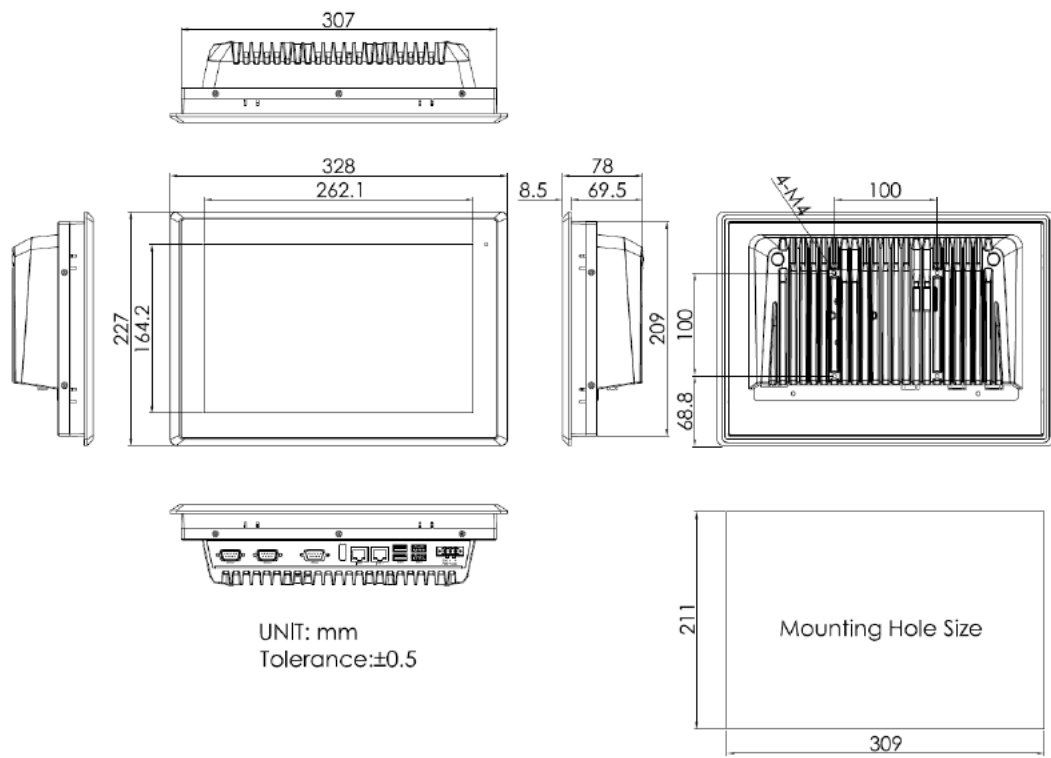
Figure 3 Dimensions of TP-7045-12 Wide
